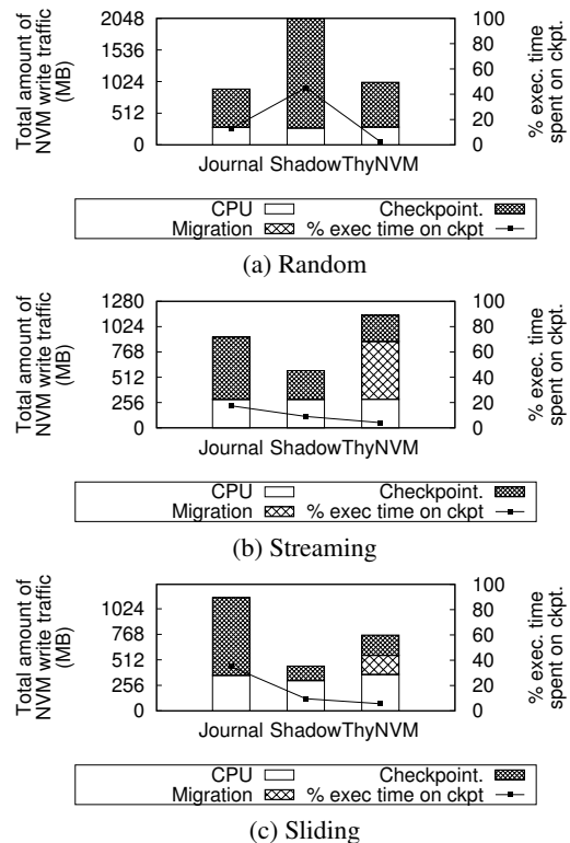
Figure 8: NVMM write traffic and checkpointing delay (% of execution time spent on checkpointing) of micro-benchmarks on different memory systems. “CPU” represents writes from CPU to NVMM, and “Checkpoint.”/“Migration” represents NVMM writes due to checkpointing/migration.
